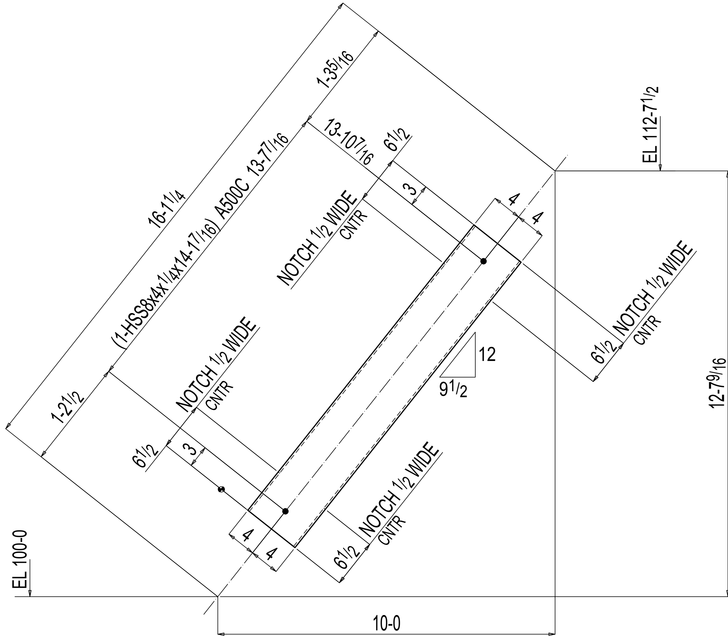
ONE VERTICAL BRACE VB3
