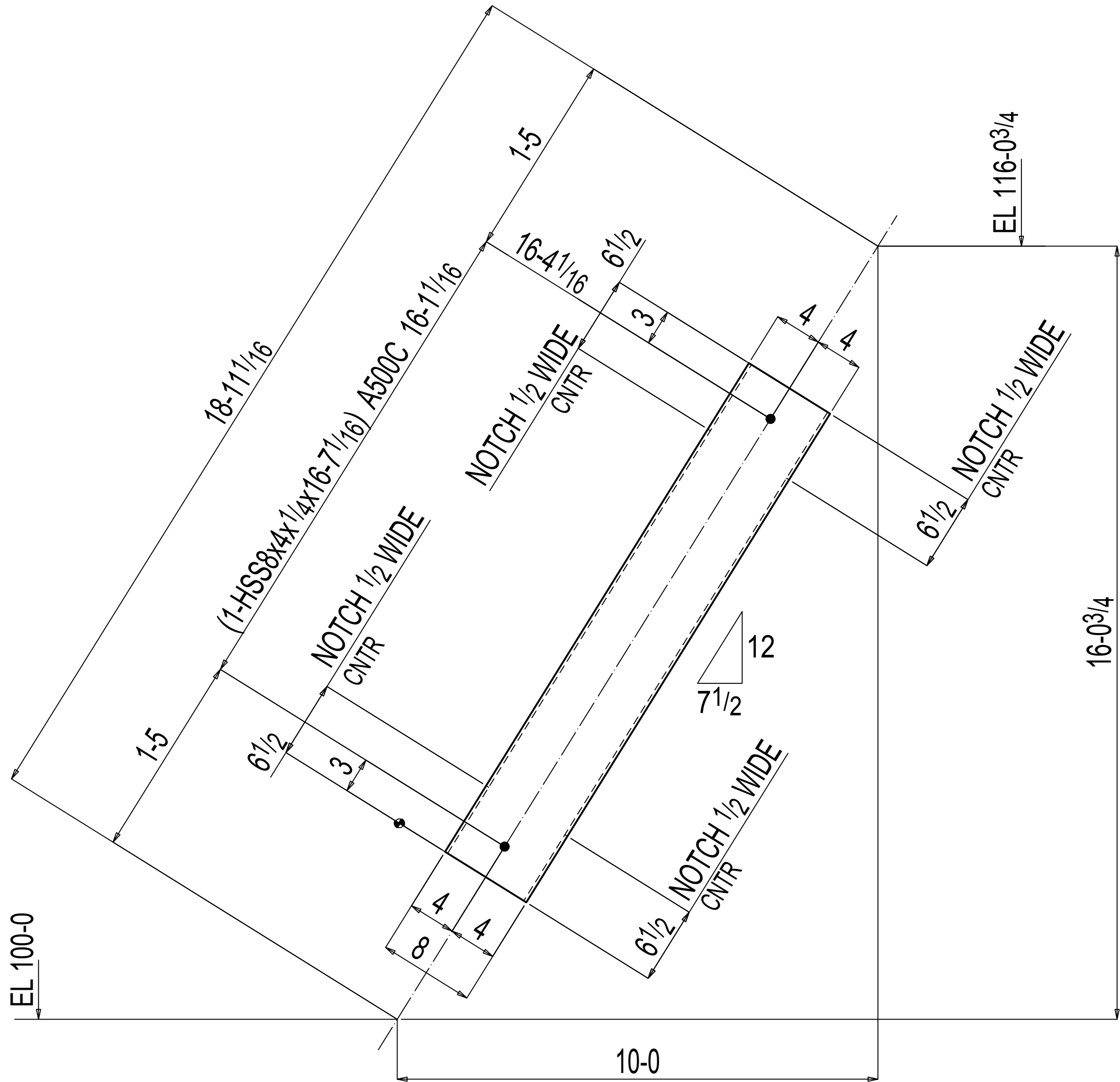
ONE VERTICAL BRACE VB2
